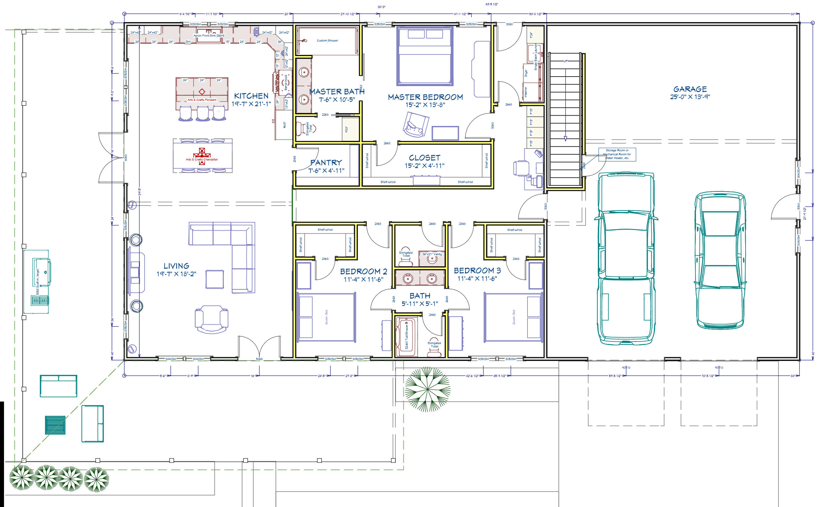
COMPLETE LAYOUT
